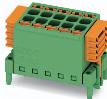
The figure shows a 5-pos. version with 10 contacts
