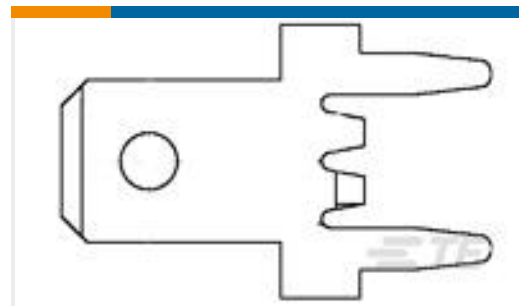
TE Part #1217332-1 187 FASTON,PCB TAB,TCBR DEG
