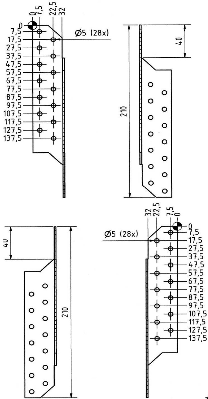
Figure A.2 Dimensions of Purlin Ties 210 right/left
