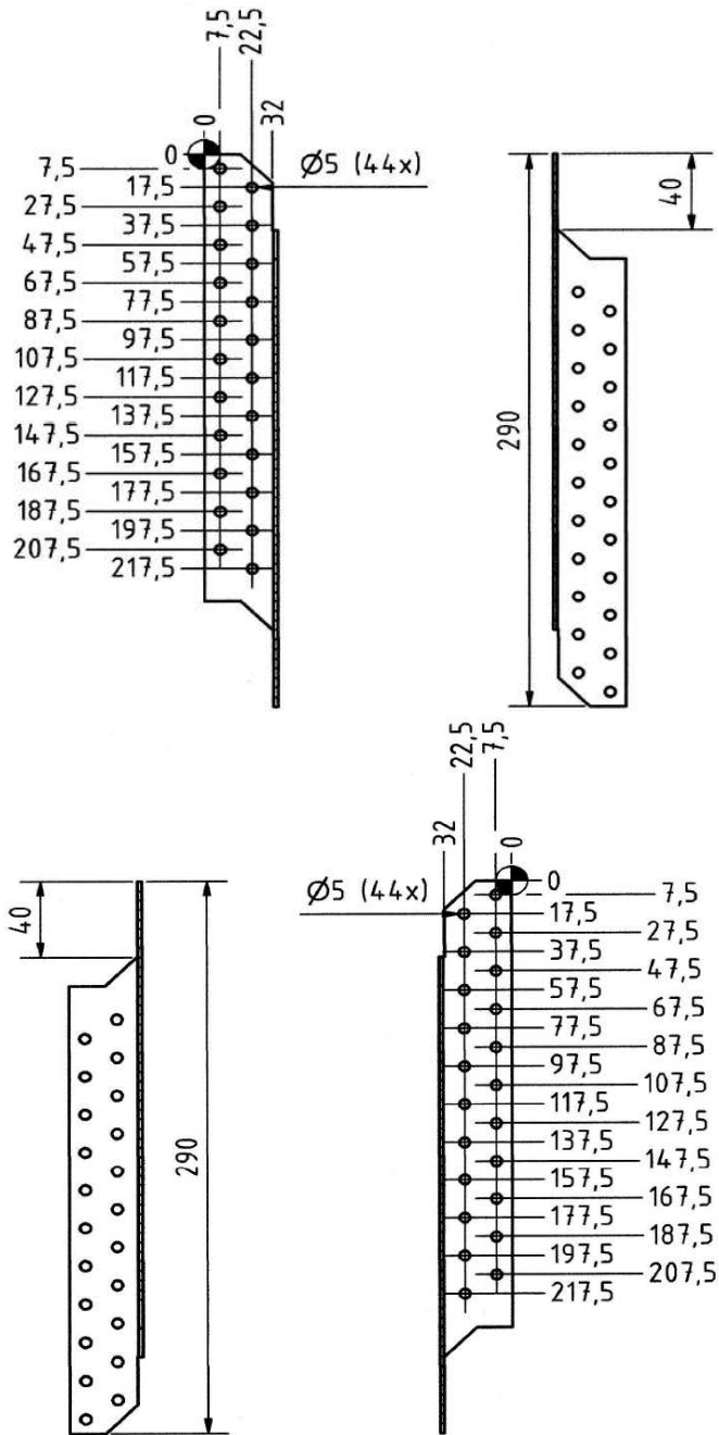
Figure A.4 Dimensions of Purlin Ties 290 right/left
