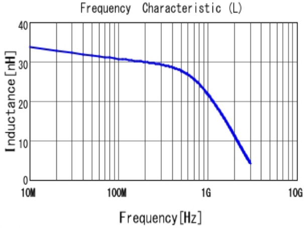
■ LQW18CA32NJ00 L
