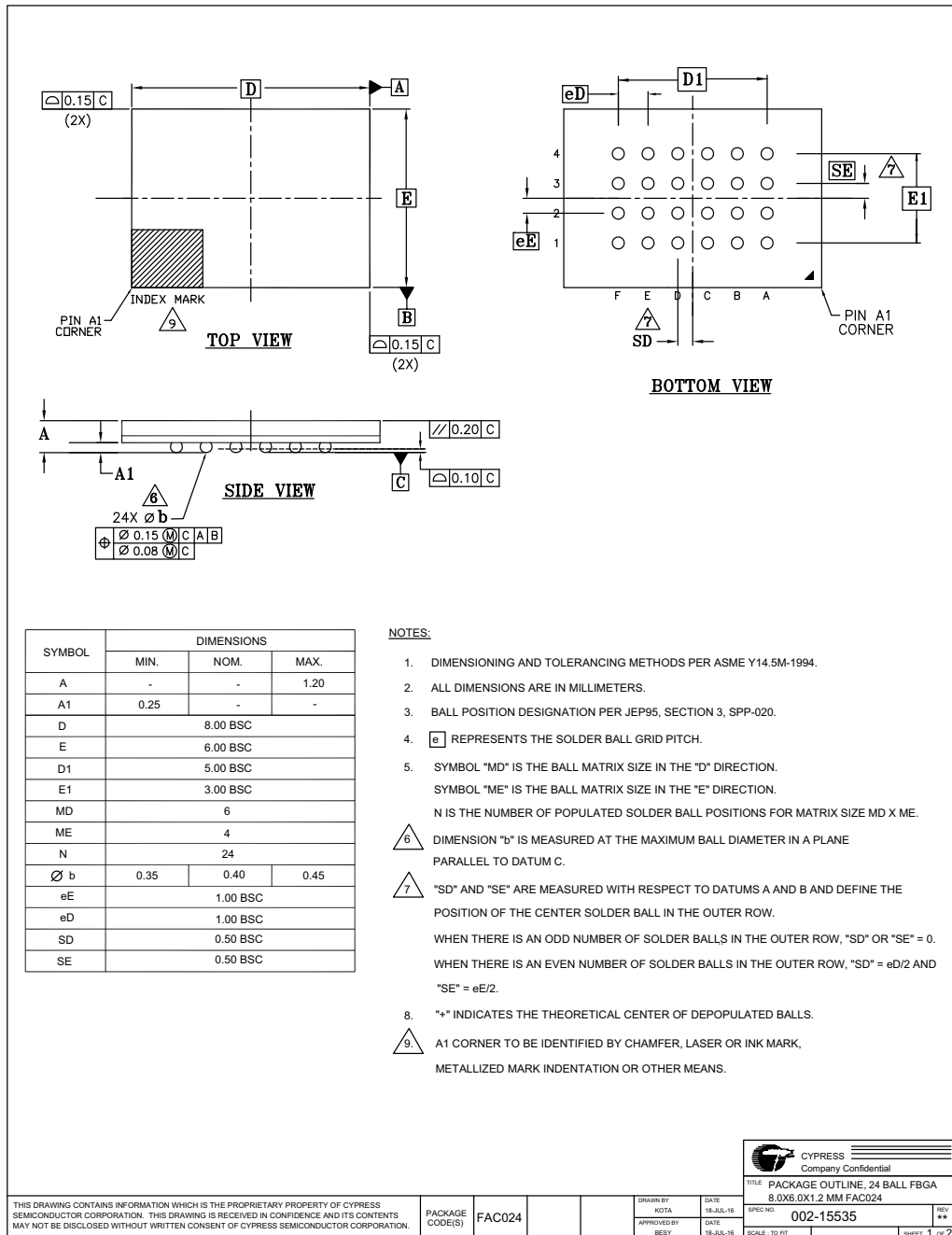
Figure 44. Ball Grid Array 24-Ball 6x8 mm (FAC024)
