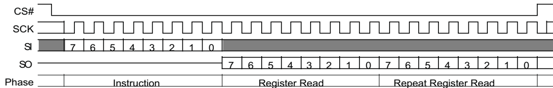
Figure 108. ASPRD Command
