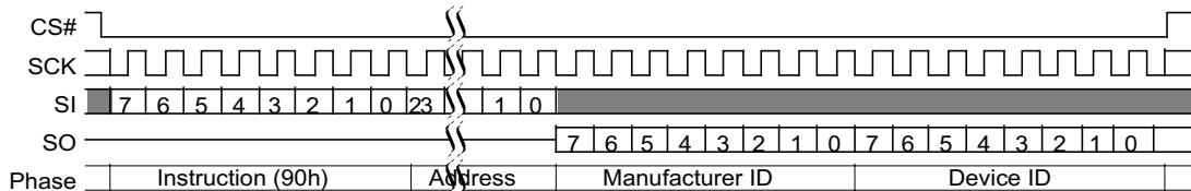
Figure 47. READ_ID (90h) Command Sequence
