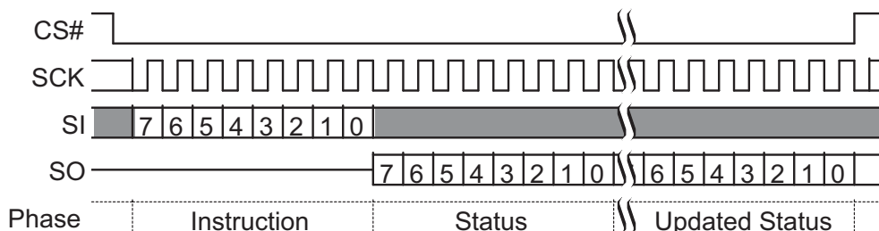
Figure 52. Read Status Register-2 (RDSR2 07h) Command Sequence
