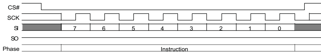
Figure 56. BRAC (B9h) Command Sequence
