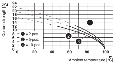
Type: TFKC 2,5/...-ST-5,08 with MSTBVA 2,5/...-G-5,08
