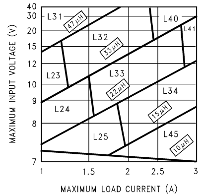
Figure 19. LM2673-5.0
