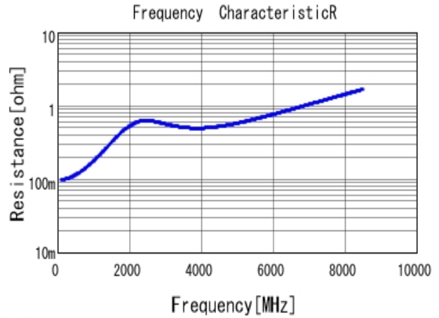
■ GRM0335C1E271GA01 R DC0V, 25degC
