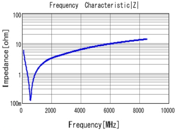
■ GRM0335C1E271GA01 |Z| DC0V, 25degC
