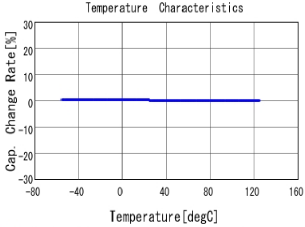
■ GRM0335C1E271GA01 C-Temp. capchange, DCOV, AC1Vrms
