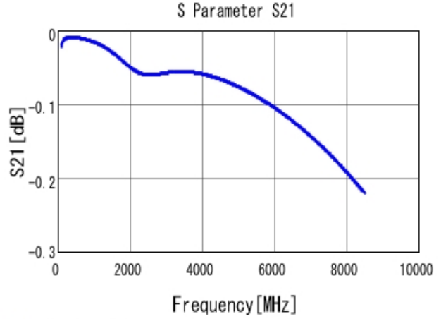
■ GRM0335C1E271GA01 S21 DCOV, 25degC
