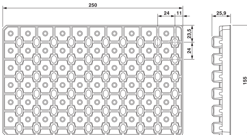
Dimensional drawing
