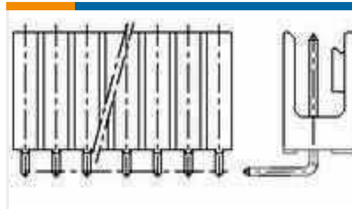
TE Teilenummer829163-5 5P MOD II SHROUDED HEADER, RT ANG.
