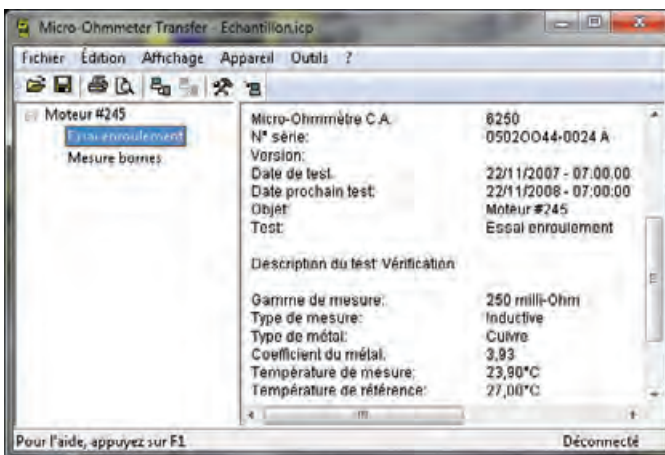
MOT MODE Results of motor winding test
