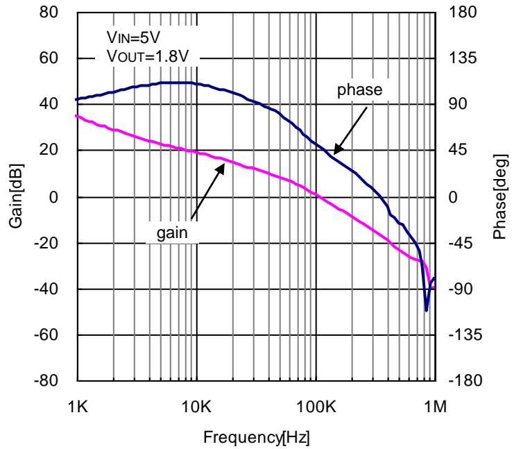
Figure 25. Closed Loop Response (VIN=5V, VOUT=1.8V, IOUT=6A, L=1.5μH, R3=6.8kΩ, C6=5600pF, C14=100pF)
