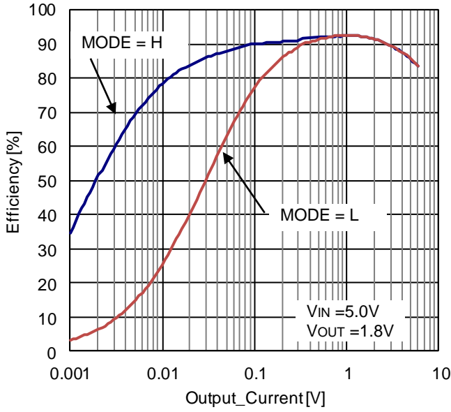
Figure 22. Efficiency vs Load Current (VIN= 5V, VOUT= 1.8V, L= 1.5μH)
