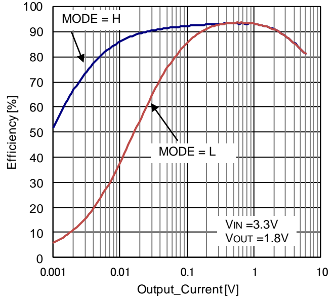
Figure 23. Efficiency vs Load Current (VIN= 3.3V, VOUT= 1.8V, L= 1.0μH)
