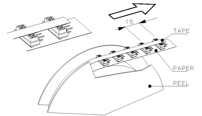
REEL PACKAGING DEREELING DIRECTION AND CONNECTOR POSITION 1500 CONNECTORS PER REEL FOR ALL PARTNUMBERS
