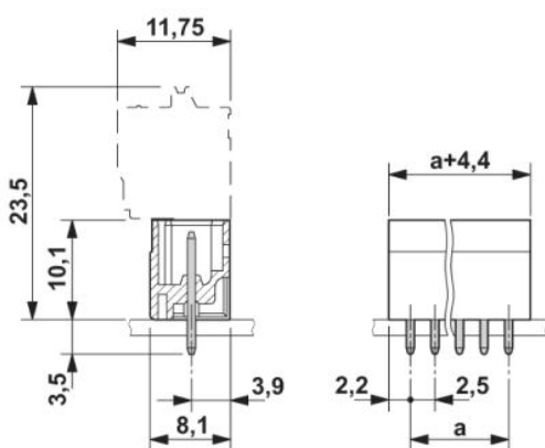
Dimensioned drawing
