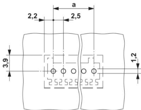
Drilling diagram
