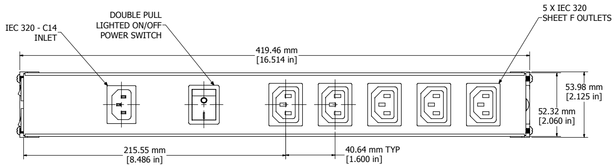
ASSEMBLY - VIEW FROM TOP
