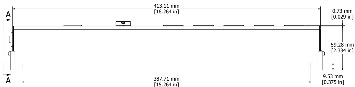
ASSEMBLY - VIEW FROM SIDE
