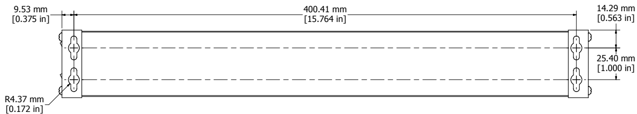
ASSEMBLY - VIEW FROM BOTTOM
