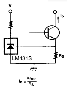
Figure 9. Constant-Current Sink
