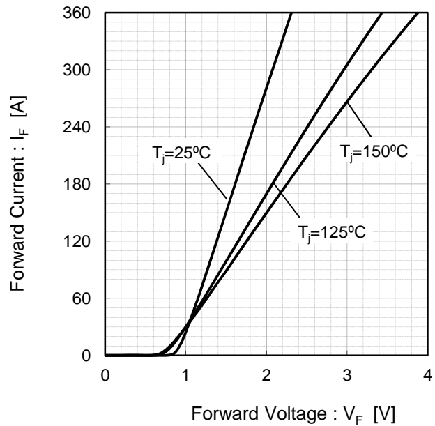
Fig.6 Forward characteristic of Diode
