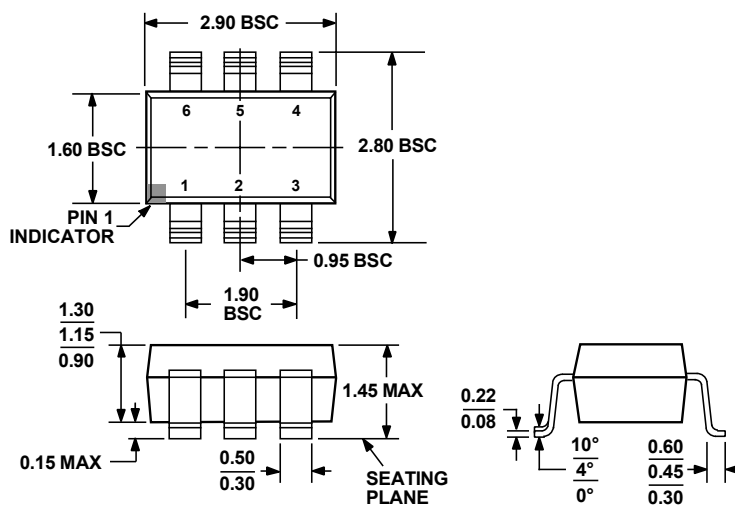
Figure 48. 6-Lead Small Outline Transistor Package [SOT-23] (RJ-6)
