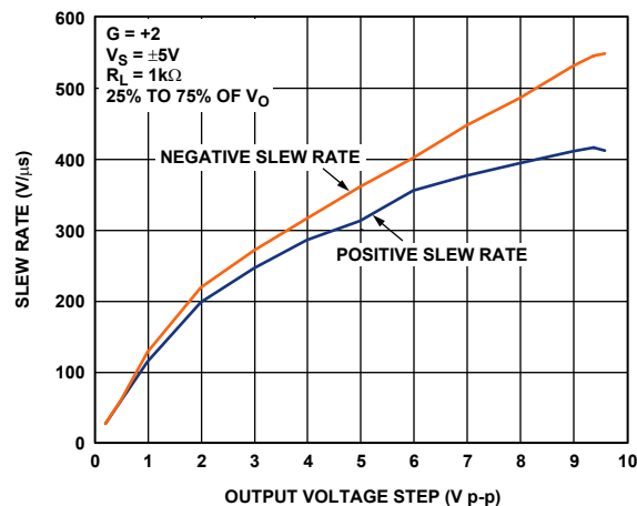
Figure 26. Slew Rate vs. Output Voltage
