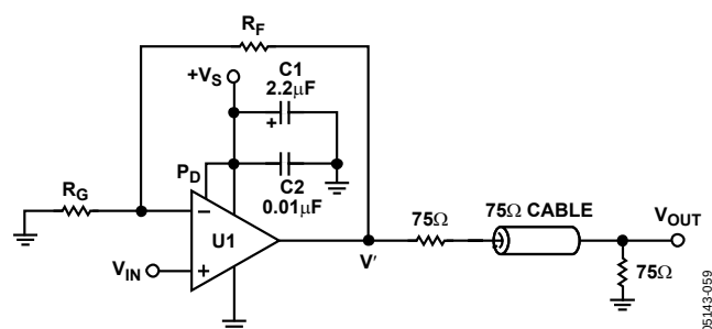
Figure 45. Video Amplifier
