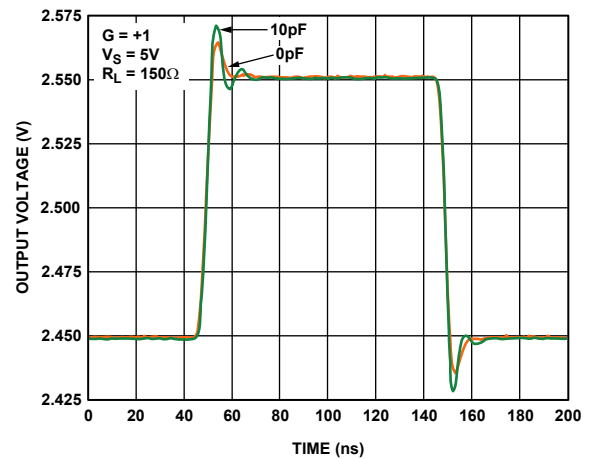
Figure 22. Small Signal Transient Response for Capacitive Load
