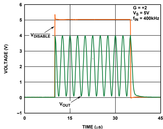
Figure 27. Enable/Disable Time
