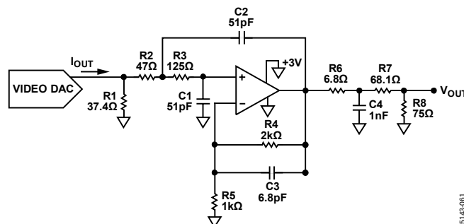
Figure 46. 8 MHz Video Reconstruction Filter Schematic
