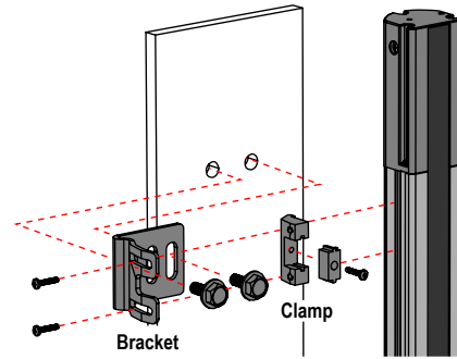
Figure 21. Side-mount hardware attachment
