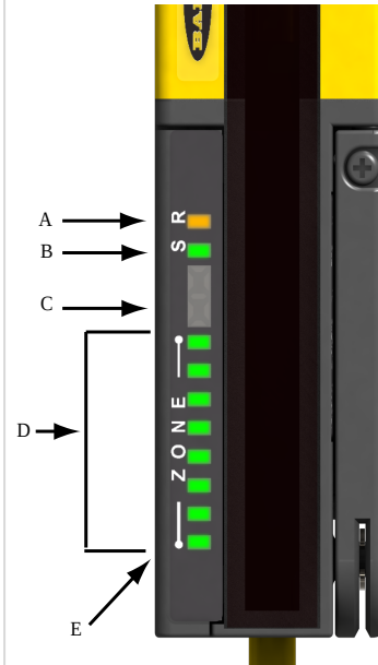
Figure 45. Receiver
