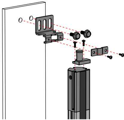
Figure 20. End-mount hardware attachment
