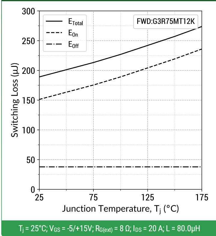
Figure 25: Inductive Switching Energy v/s Temperature ( V_{DD} = 800V )
