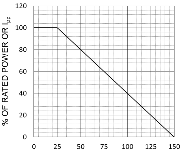
T_a (°C) POWER DERATING CURVE
