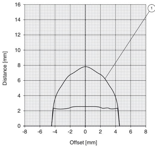
Reading range in steel IQC21-10
