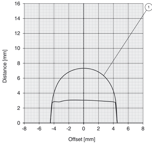
Reading range in aluminum IQC21-10
