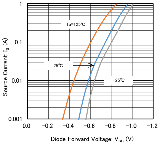
(6) Source Current vs. Diode Forward Voltage
