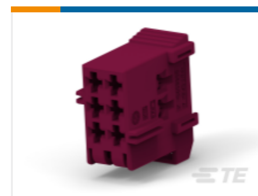
TE Part # 2355073-4 6POS,AMP MCP 2.8,REC HSG,UNSLD, COD D,VLT
