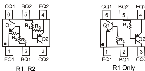
Device Schematic
