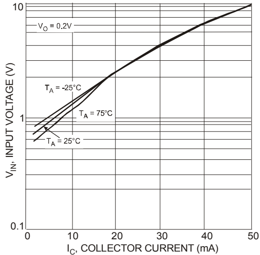
Fig. 28 Typical Input Voltage vs. Collector Current
