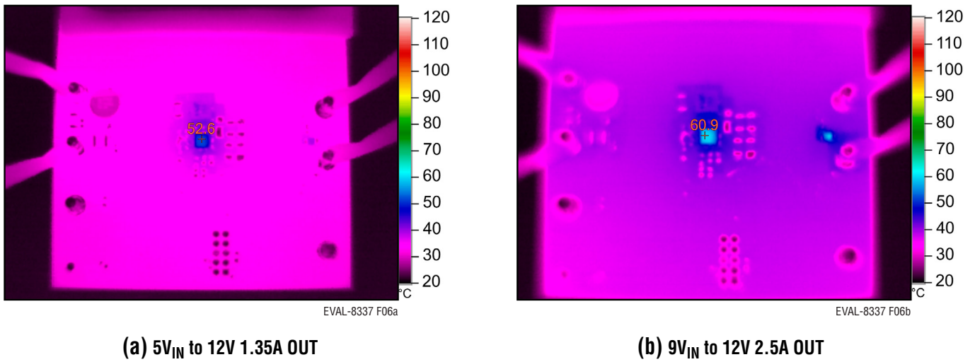
Figure 6. EVAL-LT8337-AZ Thermals
