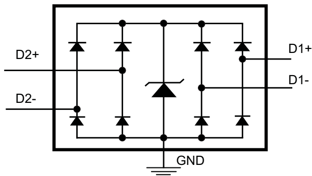
TPD4EUSB30 Circuit
