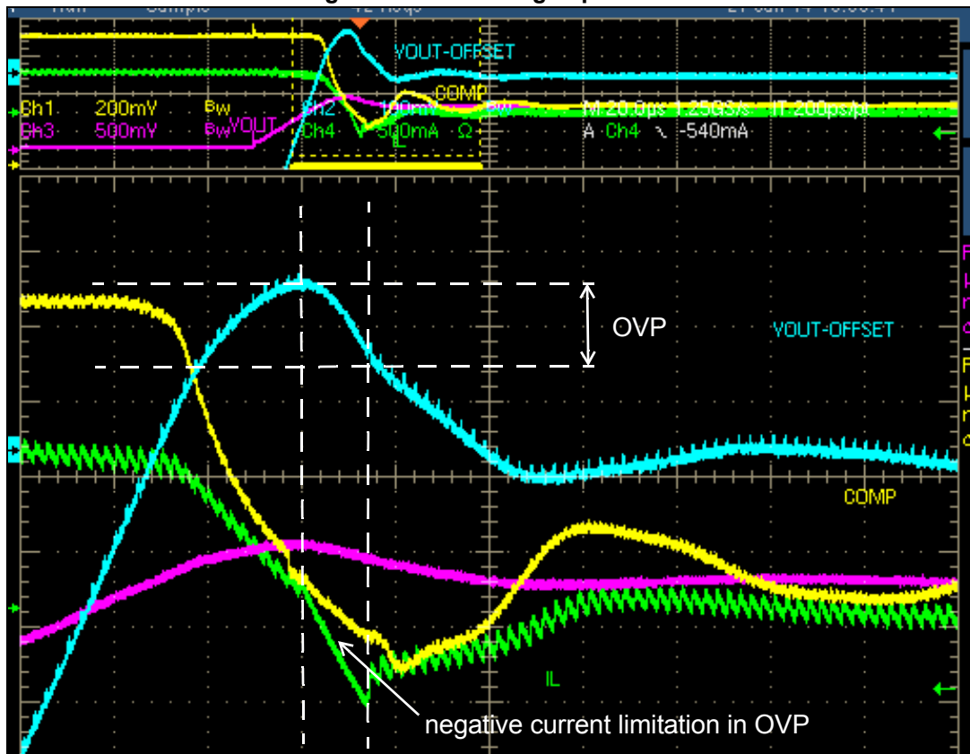
Figure 23. Overvoltage operation
