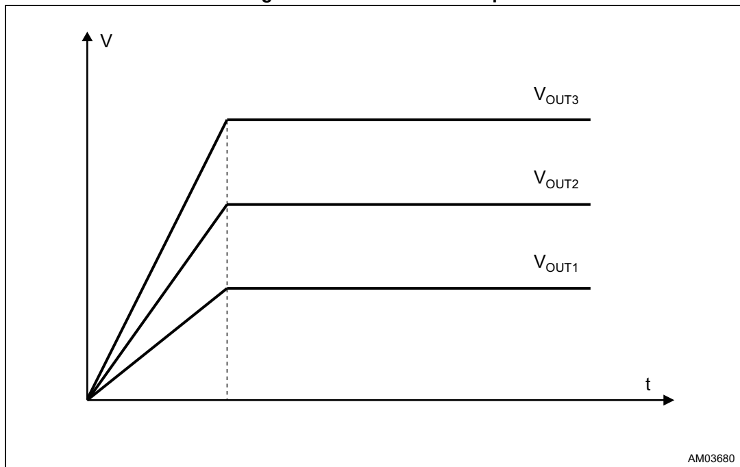
Figure 10. Ratiometric startup
