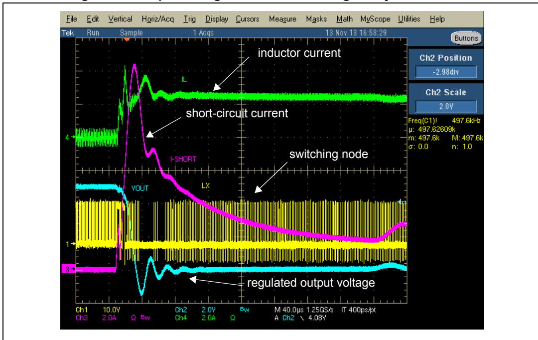
Figure 20. Output voltage oscillations during heavy short-circuit
