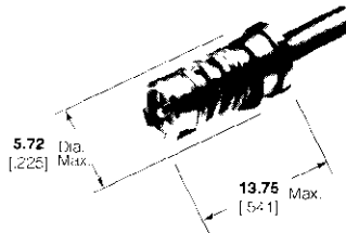
RG-405 Semi-Rigid/2.18 [.086] Cable Part No. 413249-1
