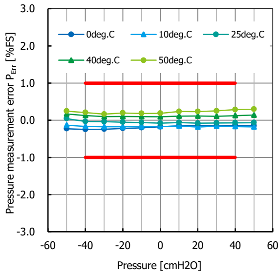
Fig. 23.3 Pressure measurement error P_{Err} temperature characteristic 0\sim 50^{\circ}\text{C}
