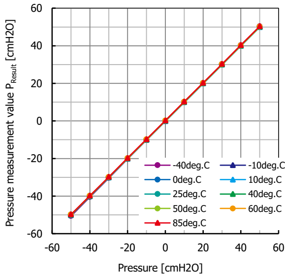
Fig. 23.1 Pressure measurement value P_{Result} temperature characteristic
