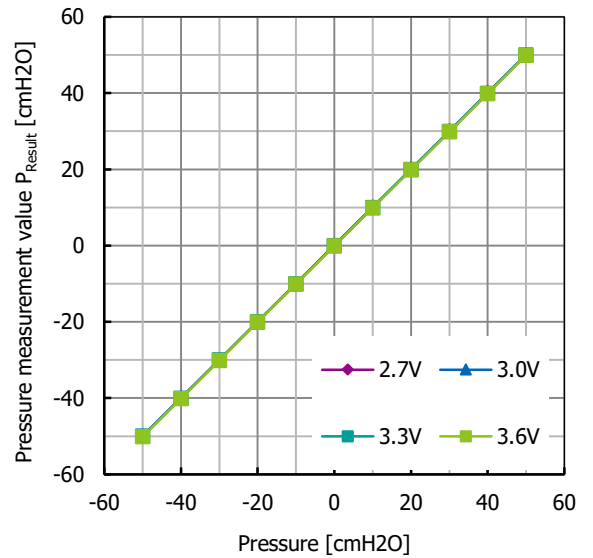
Fig. 23.2 Pressure measurement value P_{Result} supply voltage characteristic
