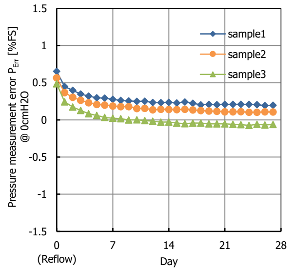
Fig. 23.8 Pressure measurement error P_{Err} @0cmH 2 O Reflow drift
