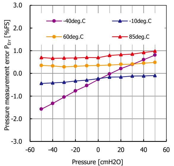
Fig. 23.4 Pressure measurement error P_{Err} temperature characteristic -40\sim 85^{\circ}\text{C}
