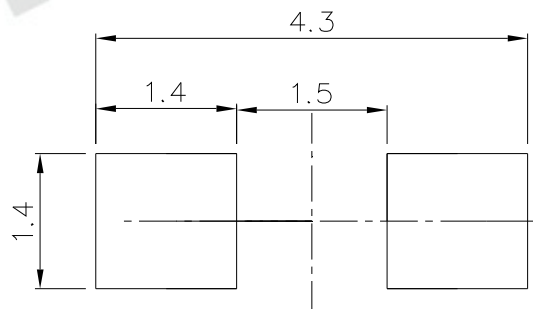
Recommended soldering pad design
