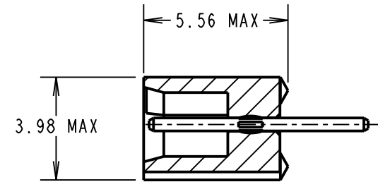
SECTION X-X
