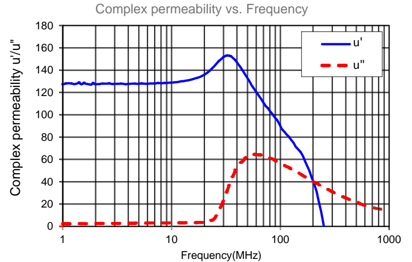
MEASURED BY ANGILENT E4991A , 1Ts .
