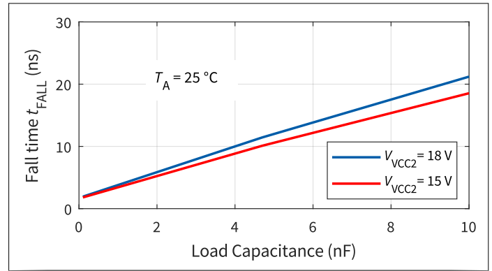
Figure 24 Fall time t_{\text{FALL}} vs. load capacitance
