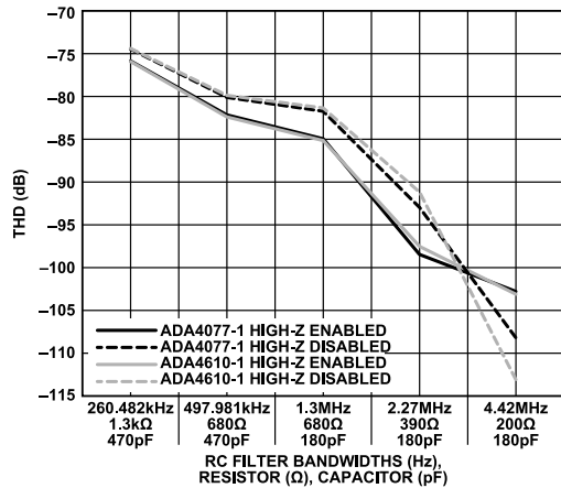
Figure 44. THD vs. RC Filter Bandwidths for Various Precision ADC Drivers for the AD4000, f_{IN} = 1 kHz (See the Typical Performance Characteristics Section for Operating Conditions )
