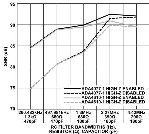
Figure 43. SNR vs. RC Filter Bandwidths for Various Precision ADC Drivers for the AD4000, f_{IN} = 1 kHz (See the Typical Performance Characteristics Section for Operating Conditions )
