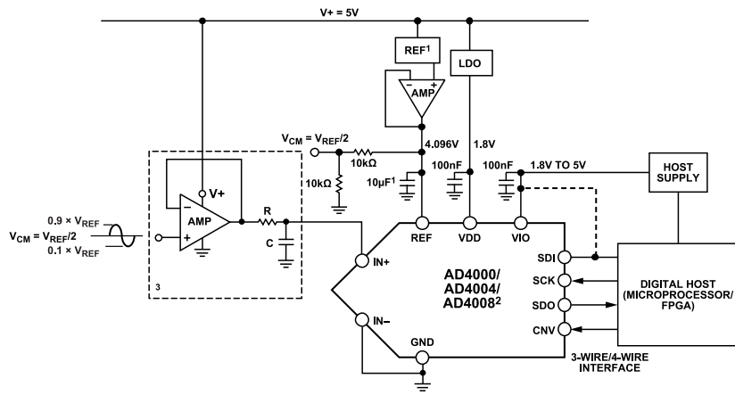
Figure 38. Typical Application Diagram with Multiple Supplies
