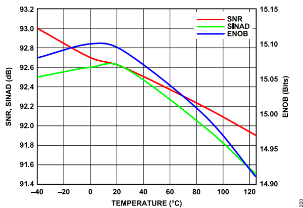
Figure 18. SNR, SINAD, and ENOB vs. Temperature, f_{IN} = 1 \text{ kHz}
