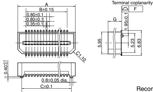
General tolerance: ±0.3
