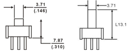
TSR-3386(STYLE)-EY5-(RESISTANCE CODE)-T
