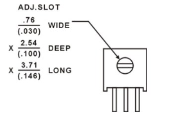
TSR-3386(STYLE)-EY5-(RESISTANCE CODE)
