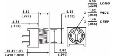
TSR-3386(STYLE)-EY5-(RESISTANCE CODE)-L
