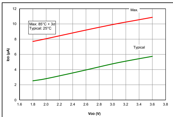
FIGURE 36-9: I_{DD} , EC Oscillator LP Mode, F_{OSC} = 32\text{ kHz} , PIC16LF1614/8 Only.
