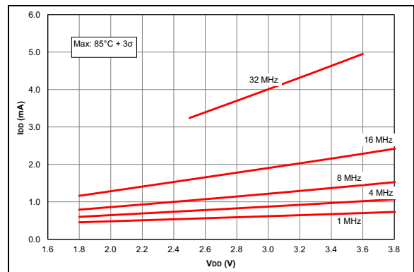
FIGURE 36-6: I_{DD} Maximum, HFINTOSC Mode, PIC16LF1614/8 Only.
