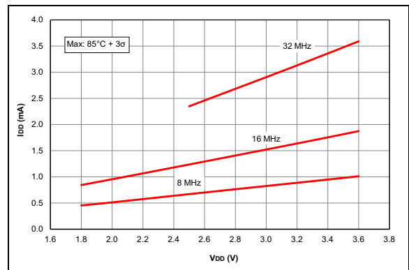
FIGURE 36-18: I_{DD} Maximum, EC Oscillator HP Mode, PIC16LF1614/8 Only.
