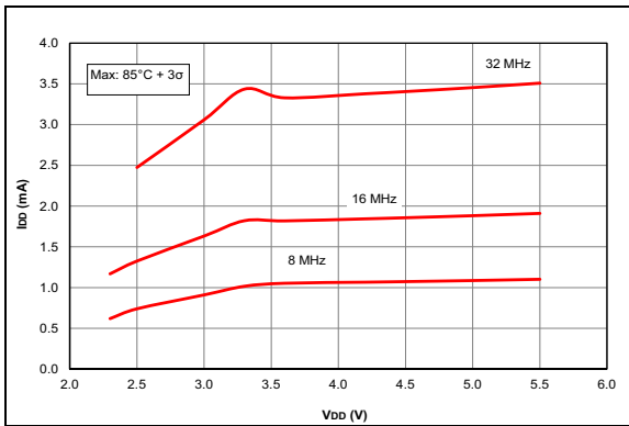
FIGURE 36-20: I_{DD} Maximum, EC Oscillator HP Mode, PIC16F1614/8 Only.
