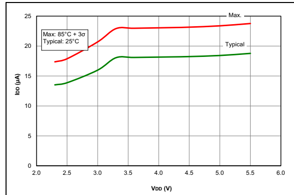
FIGURE 36-10: I_{DD} , EC Oscillator LP Mode, F_{OSC} = 32\text{ kHz} , PIC16F1614/8 Only.
