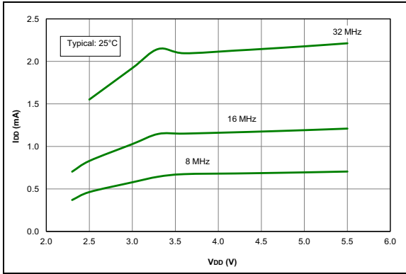
FIGURE 36-19: I_{DD} Typical, EC Oscillator HP Mode, PIC16F1614/8 Only.
