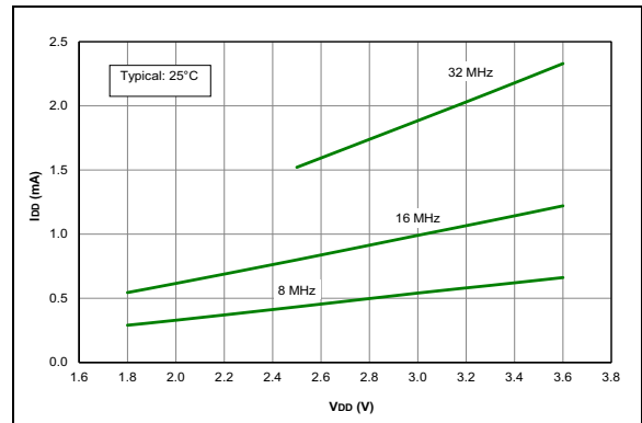
FIGURE 36-17: I_{DD} Typical, EC Oscillator HP Mode, PIC16LF1614/8 Only.
