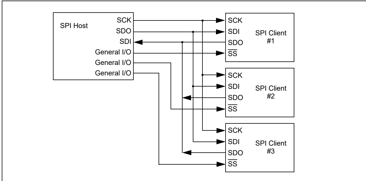
FIGURE 24-4: SPI HOST AND MULTIPLE CLIENT CONNECTION
