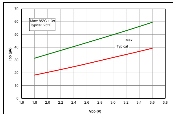
FIGURE 36-11: I_{DD} , EC Oscillator LP Mode, F_{OSC} = 500\text{ kHz} , PIC16LF1614/8 Only.
