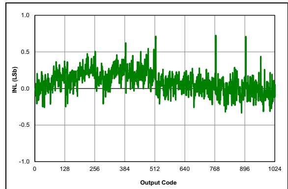
FIGURE 36-65: ADC 10-bit Mode, Single-Ended INL, V_{DD} = 3.0V , T_{AD} = 1\ \mu\text{S} , 25^\circ\text{C} .
