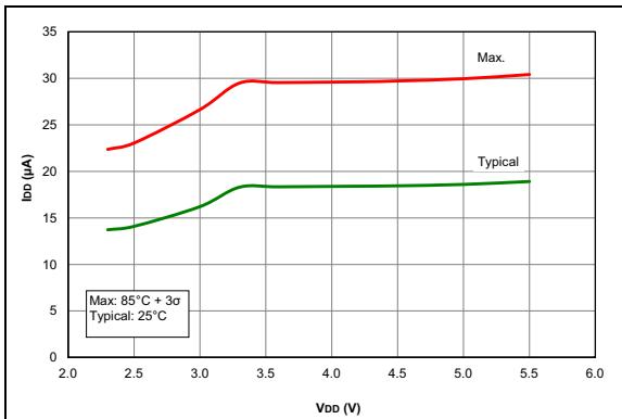
FIGURE 36-2: I_{DD} , LFINTOSC Mode, F_{OSC} = 31\text{ kHz} , PIC16F1614/8 Only.
