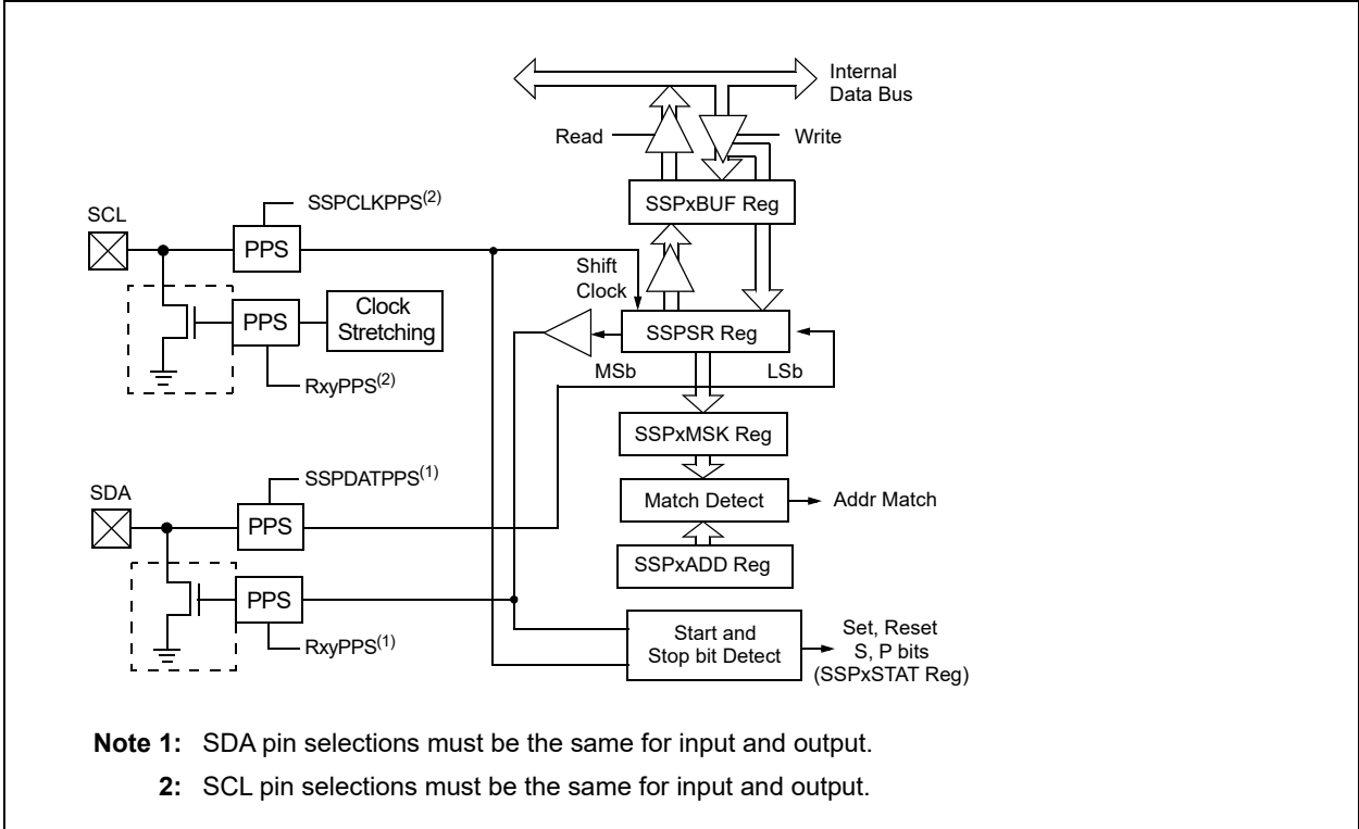
FIGURE 24-3: MSSP BLOCK DIAGRAM (I 2 C CLIENT MODE)
