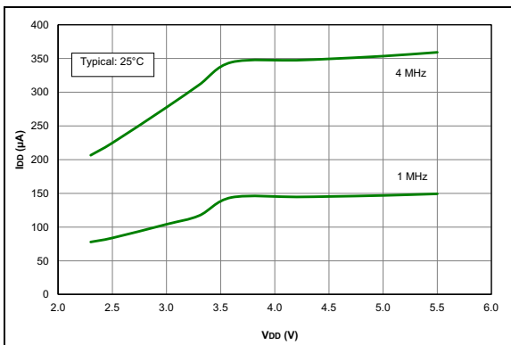
FIGURE 36-15: I_{DD} TYPICAL, EC Oscillator MP Mode, PIC16F1614/8 Only.
