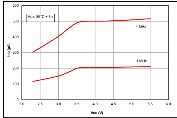
FIGURE 36-16: I_{DD} MAXIMUM, EC Oscillator MP Mode, PIC16F1614/8 Only.
