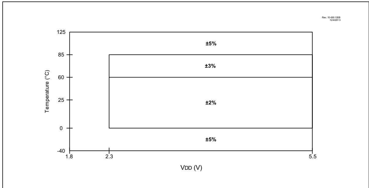
FIGURE 35-6: HFINTOSC FREQUENCY ACCURACY OVER V DD AND TEMPERATURE
