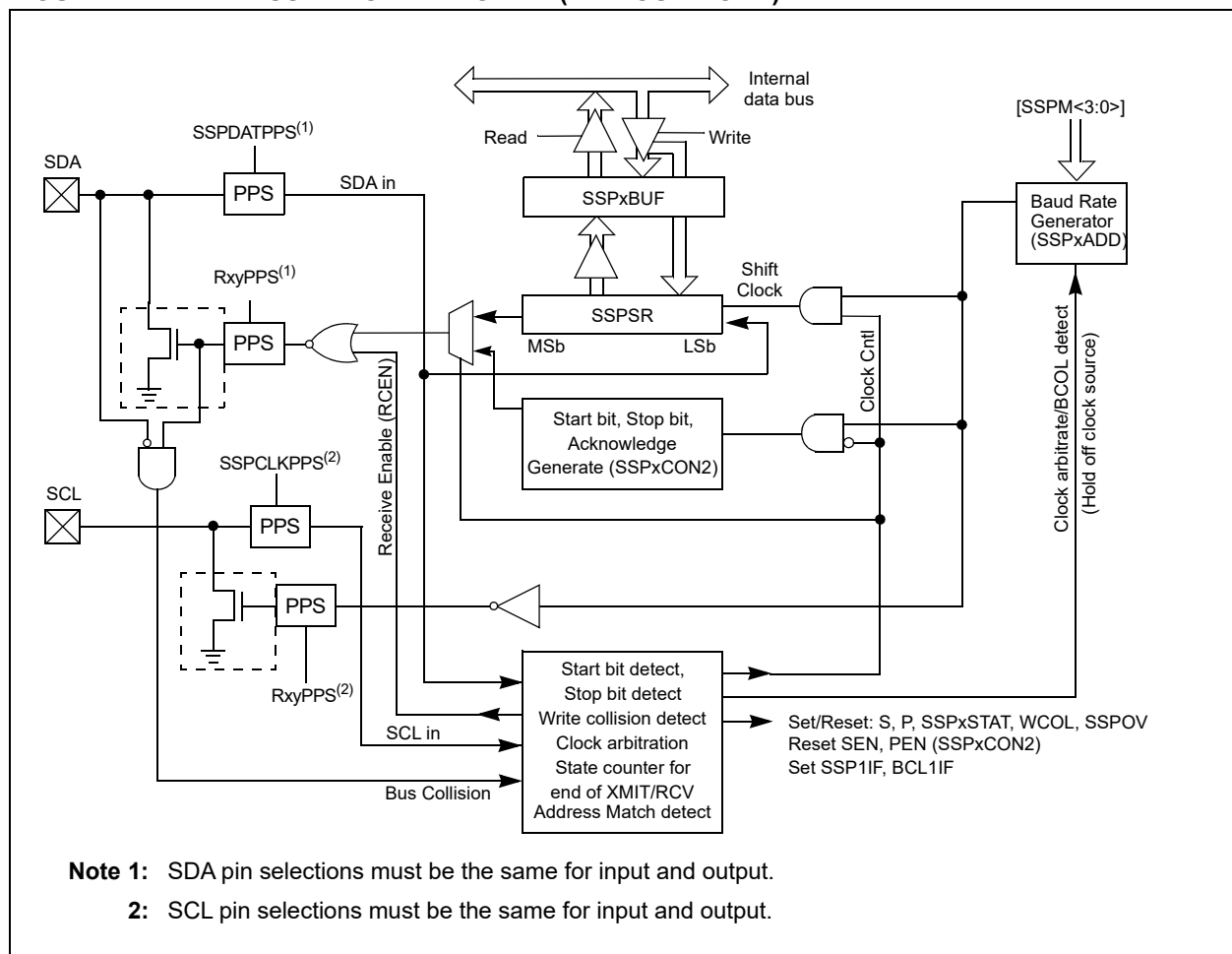
FIGURE 24-2: MSSP BLOCK DIAGRAM (I 2 C HOST MODE)
