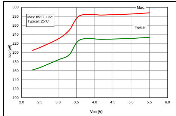
FIGURE 36-4: I_{DD} , MFINTOSC Mode, F_{OSC} = 500\text{ kHz} , PIC16F1614/8 Only.
