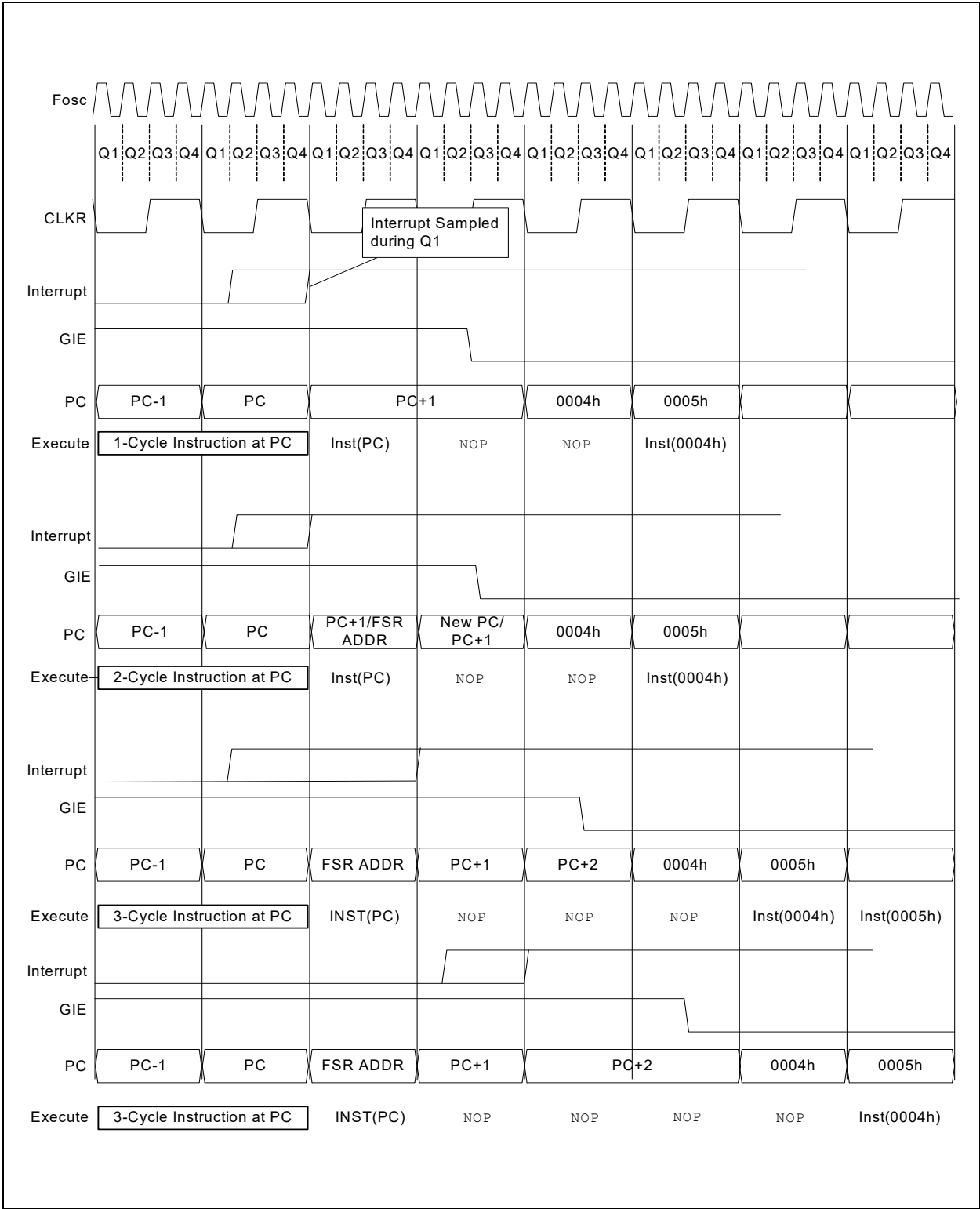
FIGURE 7-2: INTERRUPT LATENCY
