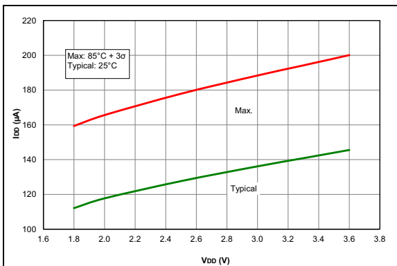
FIGURE 36-3: I_{DD} , MFINTOSC Mode, F_{OSC} = 500\text{ kHz} , PIC16LF1614/8 Only.
