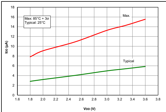
FIGURE 36-1: I_{DD} , LFINTOSC Mode, F_{OSC} = 31\text{ kHz} , PIC16LF1614/8 Only.
