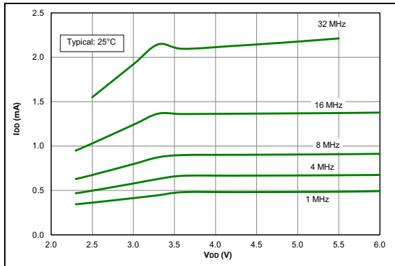
FIGURE 36-7: I_{DD} Typical, HFINTOSC Mode, PIC16F1614/8 Only.
