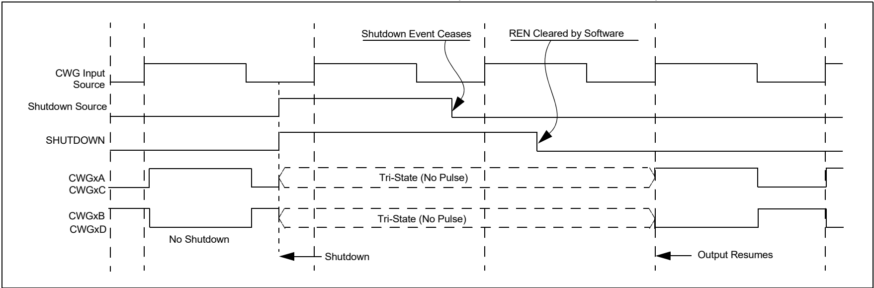
FIGURE 28-13: SHUTDOWN FUNCTIONALITY, AUTO-RESTART DISABLED (REN = 0, LSAC = 01, LSBSD = 01)
