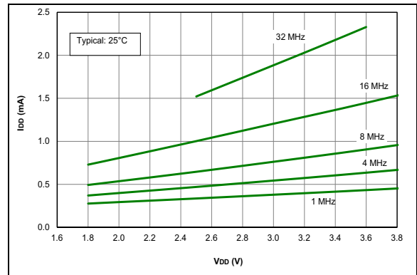
FIGURE 36-5: I_{DD} Typical, HFINTOSC Mode, PIC16LF1614/8 Only.
