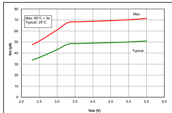
FIGURE 36-12: I_{DD} , EC Oscillator LP Mode, F_{OSC} = 500\text{ kHz} , PIC16LF1614/8 Only.
