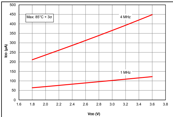
FIGURE 36-14: I_{DD} MAXIMUM, EC Oscillator MP Mode, PIC16LF1614/8 Only.
