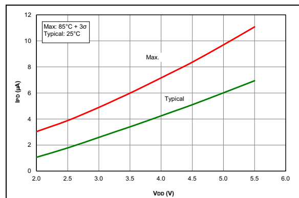
FIGURE 36-30: IPD , Timer1 Oscillator, Fosc = 32 kHz, PIC16F1614/8 Only.
