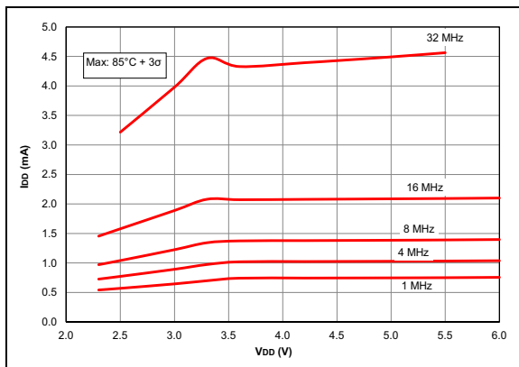
FIGURE 36-8: I_{DD} Maximum, HFINTOSC Mode, PIC16F1614/8 Only.
