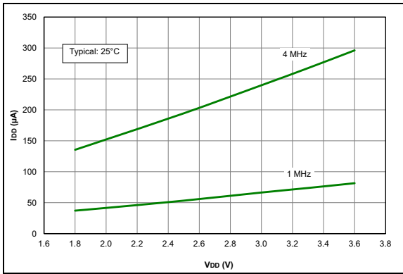
FIGURE 36-13: I_{DD} TYPICAL, EC Oscillator MP Mode, PIC16LF1614/8 Only.
