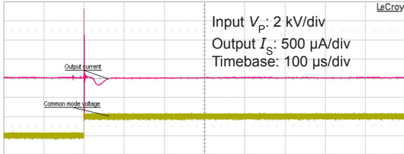
Figure 11: Typical common mode perturbation (2000 V step with 6 kV/μs, R_M = 100 \Omega )
