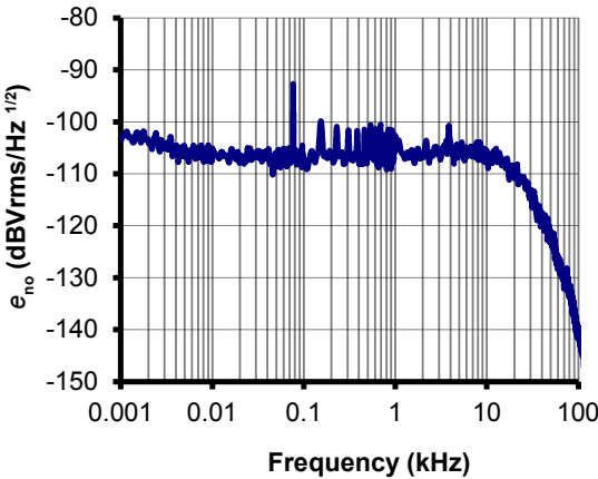
Figure 13: Typical noise voltage density of e_{no} with R_M = 50 \Omega
