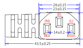
FM-302L (IEC 60320, C13, RA, 10A 125V~) (Dimensions of Connector Face)
