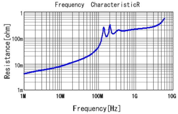
GCM1885C1H103JA16 R DCOV, 25degC
