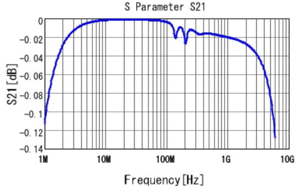
■ GCM1885C1H103JA16 S21 DCOV, 25degC
