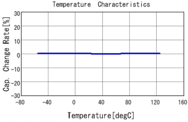
■ GCM1885C1H103JA16 C-Temp. capchange, DCOV, AC1Vrms
