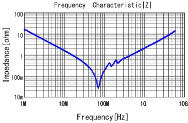
GCM1885C1H103JA16 |Z| DCOV, 25degC
