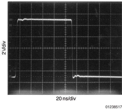
FIGURE 3. Properly Terminated Signal
