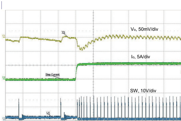
Fig. 50 - Load Step, 0.1 A to 6 A, 1 A/ \mu s, t = 10\text{ }\mu s/div Skip Mode Enabled
