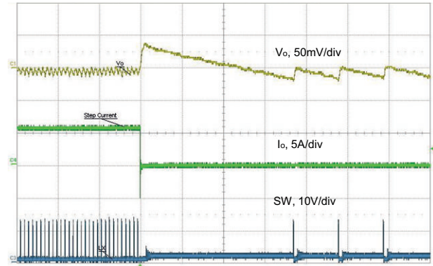
Fig. 53 - Load Release, 6 A to 0.1 A, 1 A/ \mu s, t = 20\text{ }\mu s/div Skip Mode Enabled
