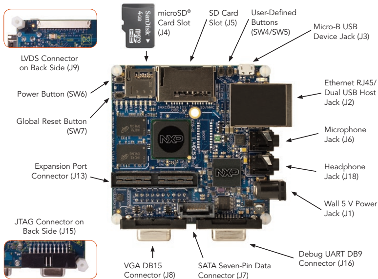
Figure 1: Top View of the i.MX53 Quick Start Board without the HDMI Module.
