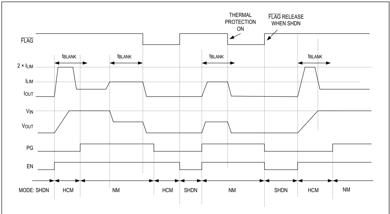
Figure 4. Latchoff
