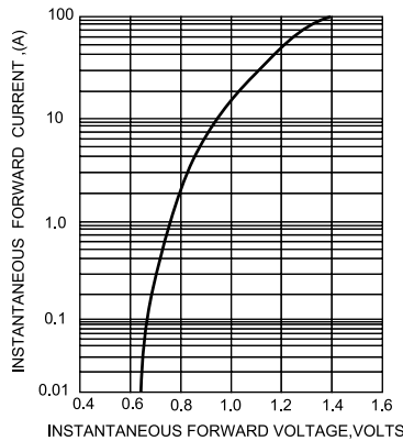
FIG.3-TYPICAL FORWARD CHARACTERISTICS
