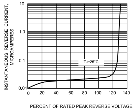
FIG.4-TYPICAL REVERSE CHARACTERISTICS
