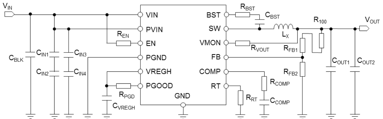
Figure 44. Reference Circuit 2
