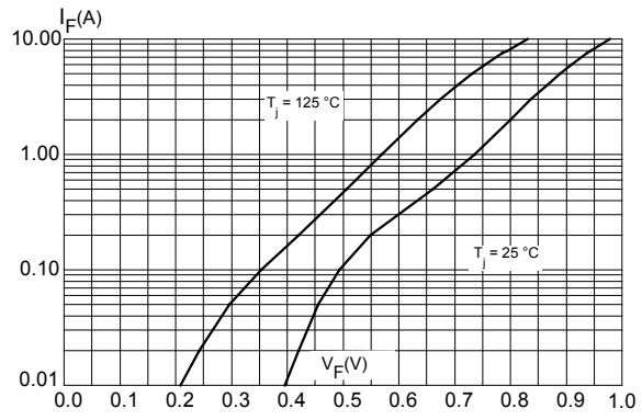
Figure 10. Forward voltage drop versus forward current (maximum values)
