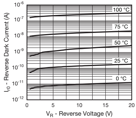
Fig. 7 - Dark Current vs. Reverse Voltage
