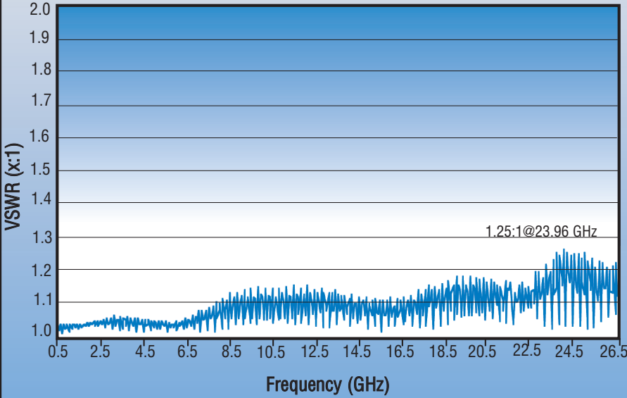
(26.5 GHz SMA Male/SMA Male, 3 ft long)
